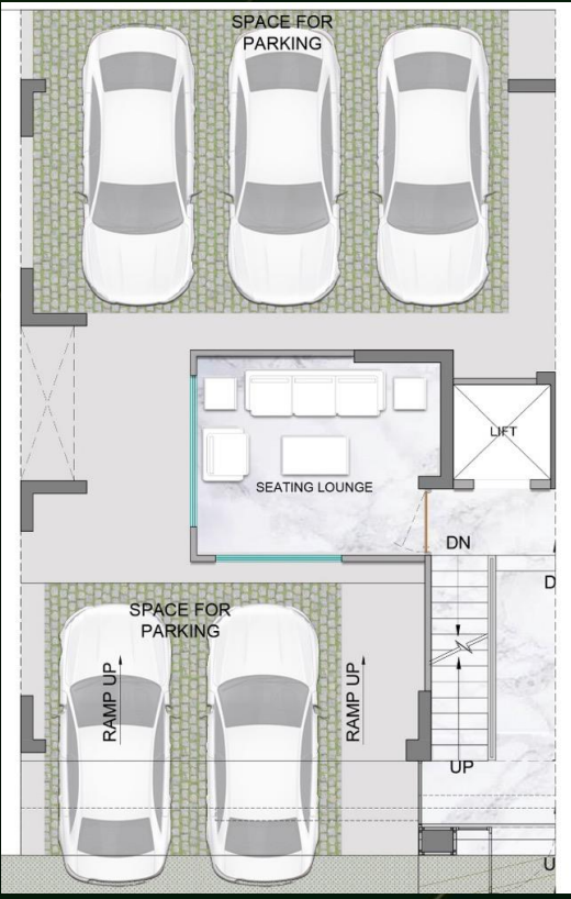
STILT FLOOR
